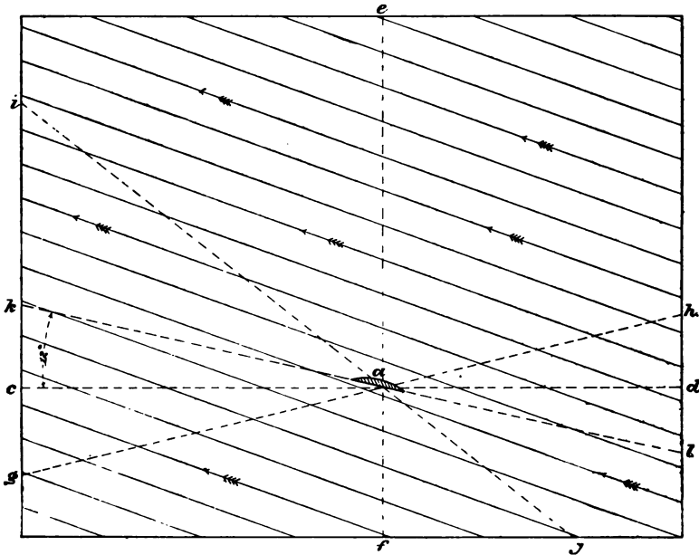
Fig. 67.—In this drawing a represents an aeroplane, or a bird's wing. Suppose that the wind is blowing in the direction of the arrows; the real path of the bird as relates to the air is from i to j ,—that is, the bird is falling as relates to the air although moving on the line c, d , against the wind. In some cases, a bird is able to travel along the line g, h , instead of in a horizontal direction, thus rising and apparently flying into the teeth of the wind at the same time.
